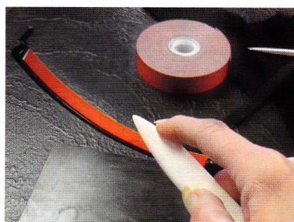
Industrial strength, high-tack sponge adhesive was used to line the curved support. The tape is aligned and burnished with bone for full adhesive activation.
